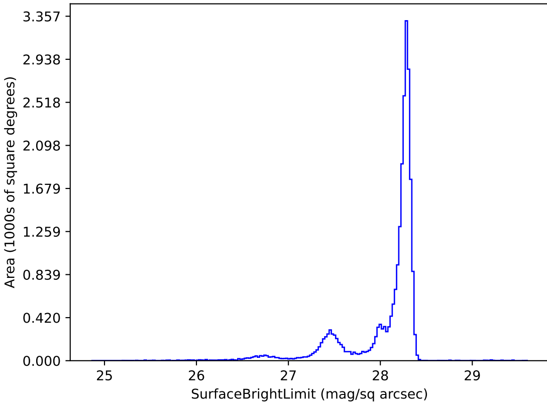
ddf_loaded_fl1_v3.4_10yrs y: SurfaceBrightLimit
