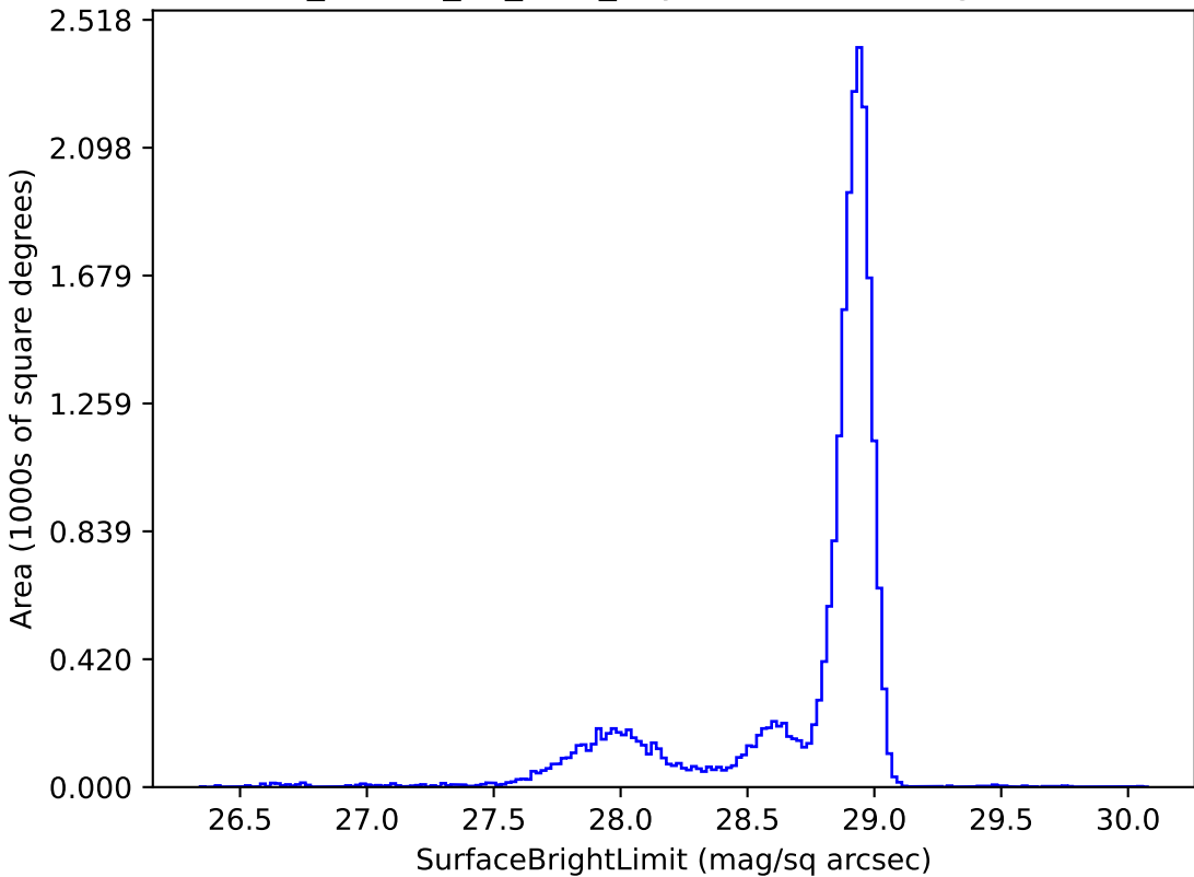
ddf_loaded_fl1_v3.4_10yrs u: SurfaceBrightLimit
