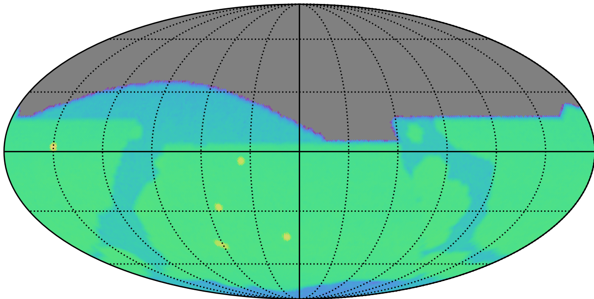
ddf_loaded_fl1_v3.4_10yrs r: SurfaceBrightLimit
