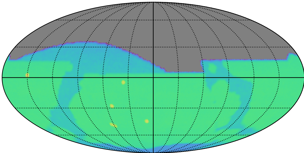
ddf_loaded_fl1_v3.4_10yrs i: SurfaceBrightLimit
