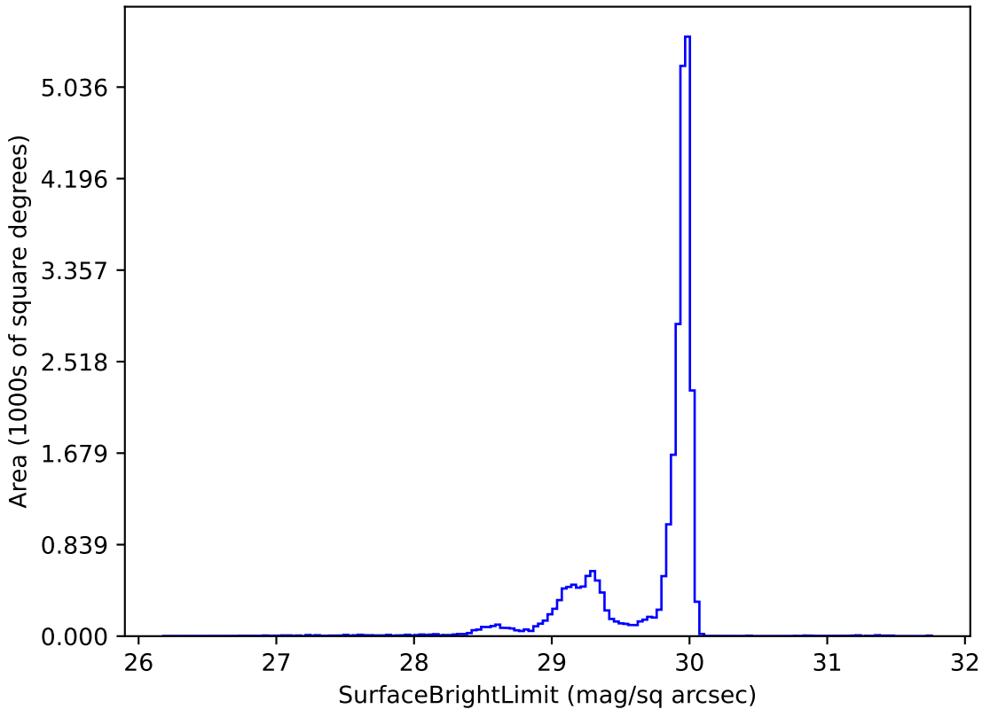
ddf_loaded_fl1_v3.4_10yrs i: SurfaceBrightLimit
