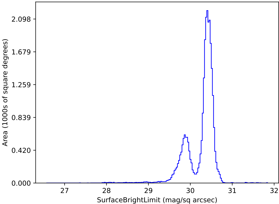
ddf_loaded_fl1_v3.4_10yrs g: SurfaceBrightLimit
