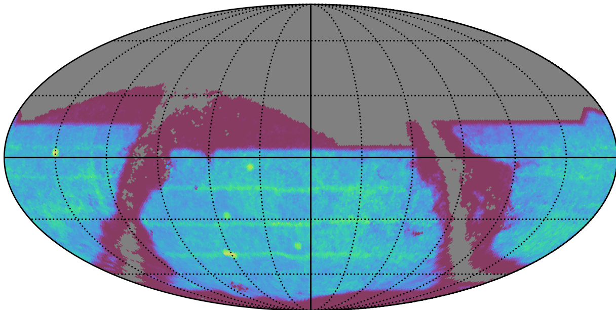
ddf_loaded_fl1_v3.4_10yrs : SNSLMetric
