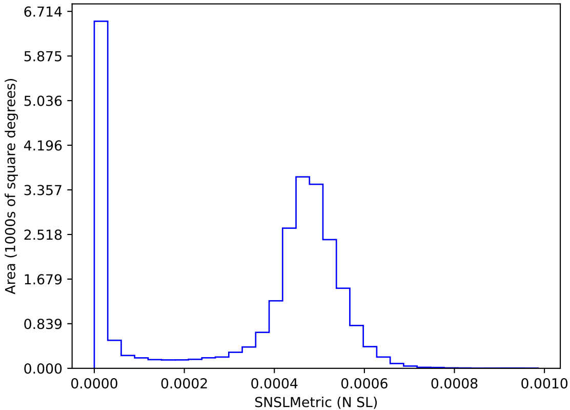
ddf_loaded_fl1_v3.4_10yrs : SNSLMetric
