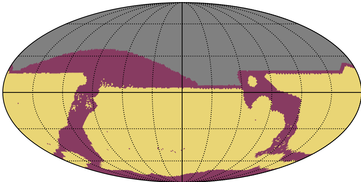
ddf_loaded_fl1_v3.4_10yrs : RapidRevisits
