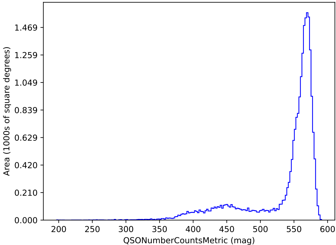
ddf_loaded_fl1_v3.4_10yrs y band and non-DD: QSONumberCountsMetric
