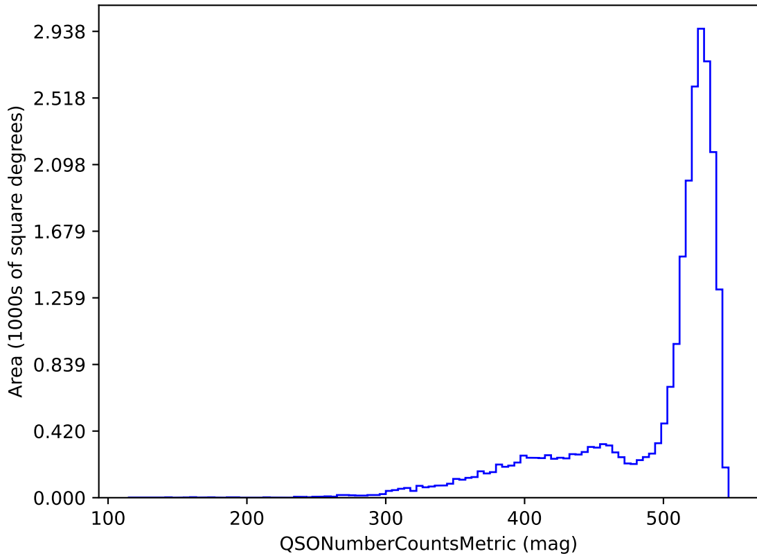
ddf_loaded_fl1_v3.4_10yrs r band and non-DD: QSONumberCountsMetric
