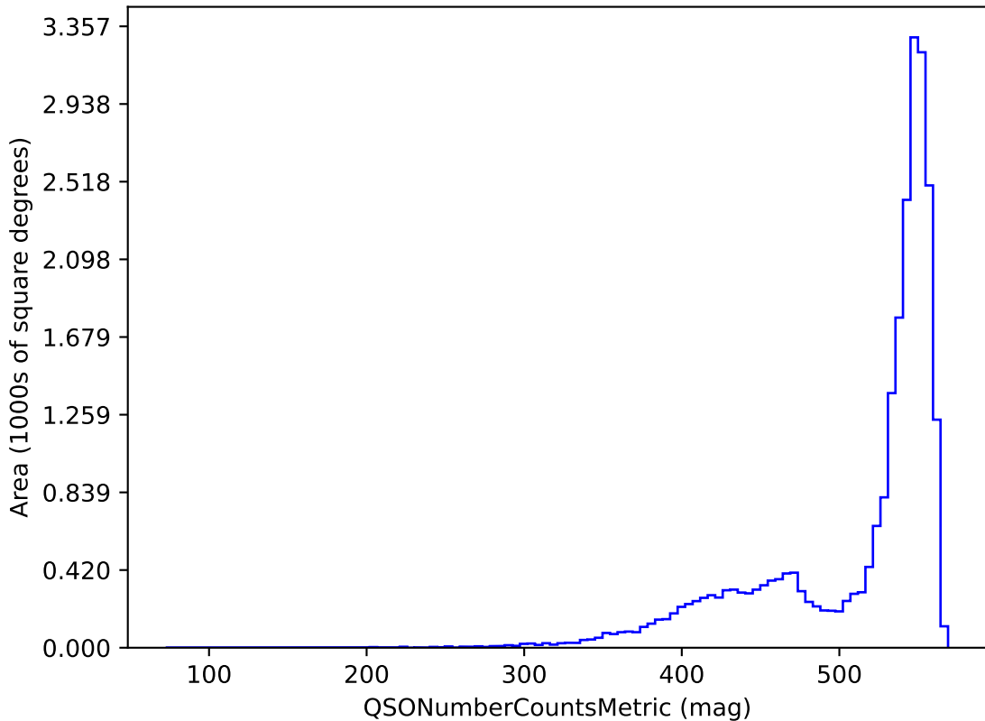
ddf_loaded_fl1_v3.4_10yrs i band and non-DD: QSONumberCountsMetric
