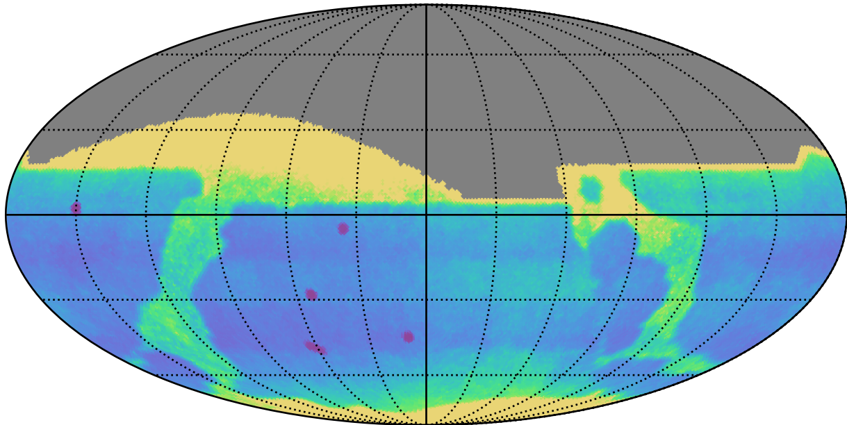
ddf_loaded_fl1_v3.4_10yrs : Proper Motion Uncert @ 24.0
