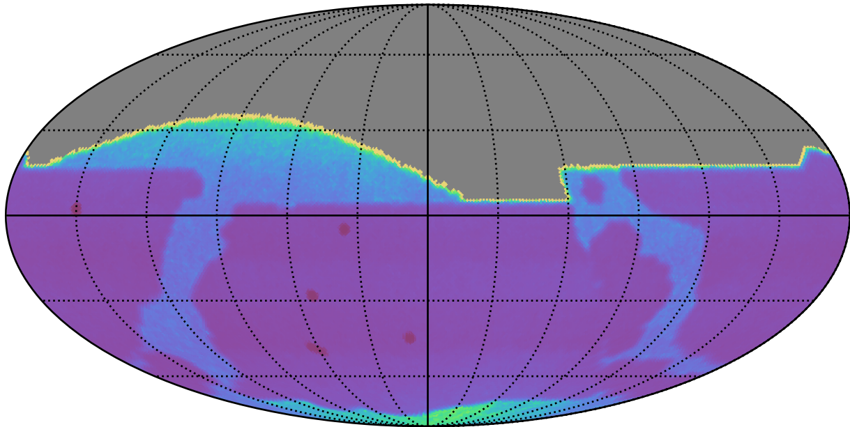
ddf_loaded_fl1_v3.4_10yrs : Proper Motion Uncert @ 20.5
