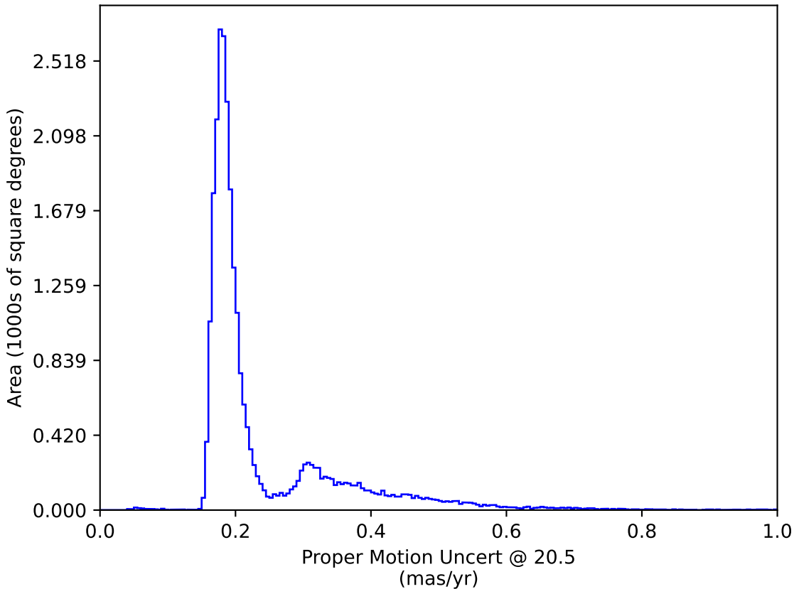
ddf_loaded_fl1_v3.4_10yrs : Proper Motion Uncert @ 20.5
