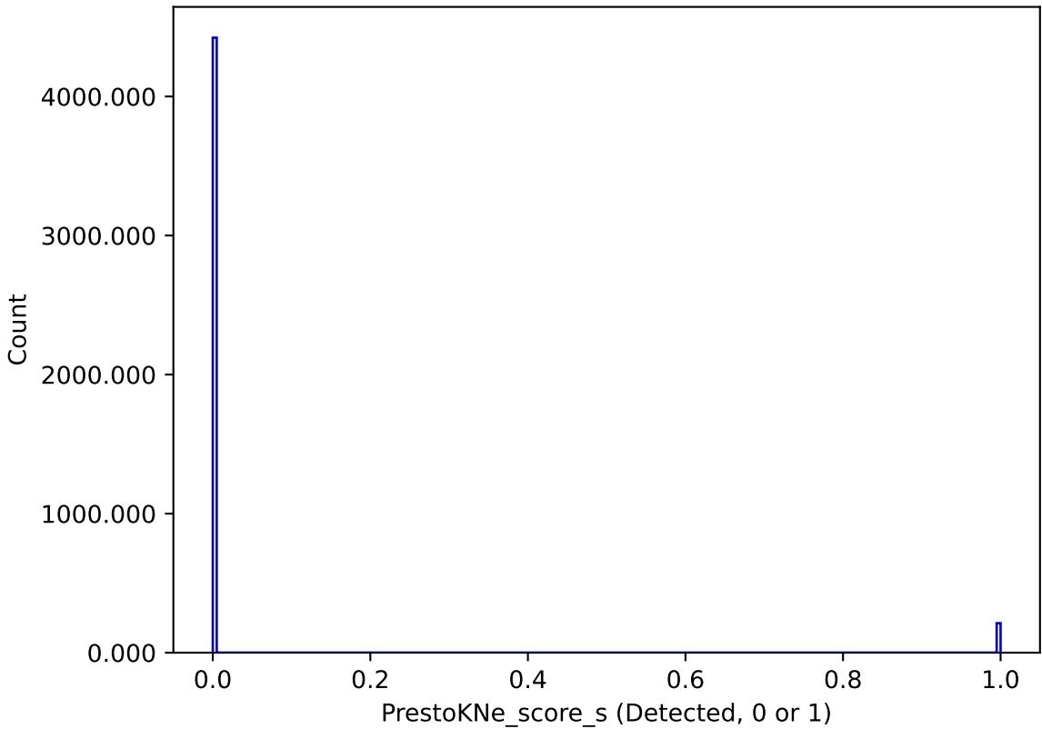
ddf_loaded_fl1_v3.4_10yrs : PrestoKNe_score_s
