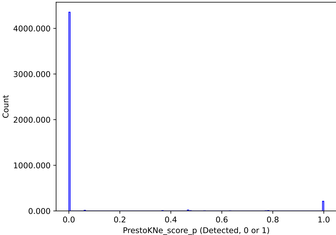
ddf_loaded_fl1_v3.4_10yrs : PrestoKNe_score_p
