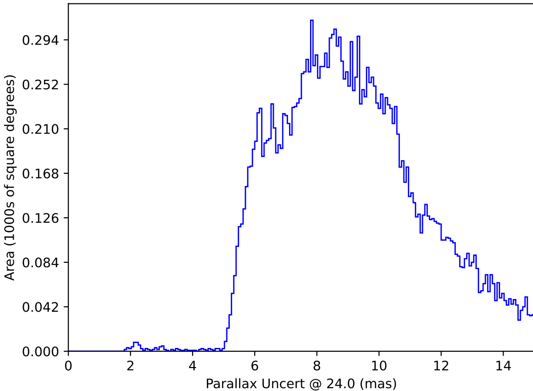
ddf_loaded_fl1_v3.4_10yrs : Parallax Uncert @ 24.0
