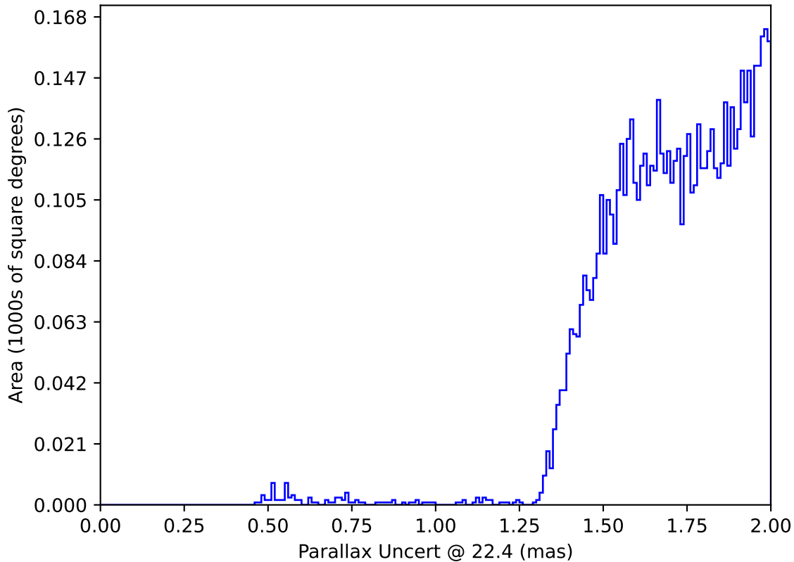
ddf_loaded_fl1_v3.4_10yrs : Parallax Uncert @ 22.4
