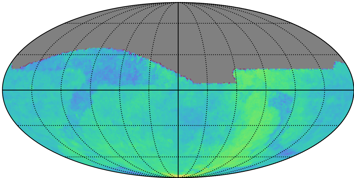
ddf_loaded_fl1_v3.4_10yrs : Parallax Coverage @ 24.0
