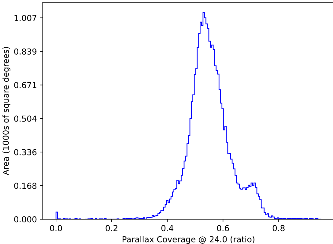
ddf_loaded_fl1_v3.4_10yrs : Parallax Coverage @ 24.0
