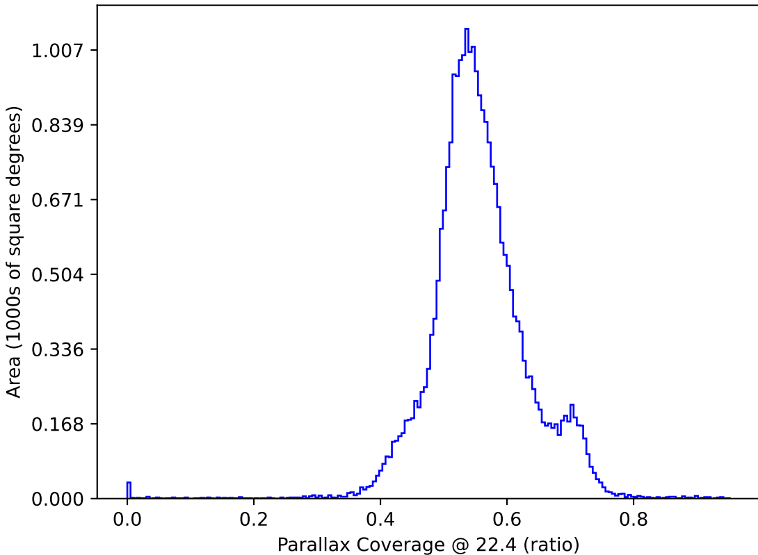
ddf_loaded_fl1_v3.4_10yrs : Parallax Coverage @ 22.4
