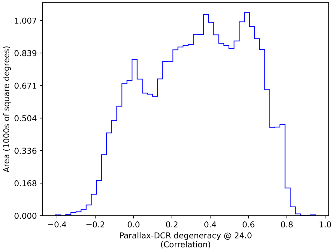
ddf_loaded_fl1_v3.4_10yrs : Parallax-DCR degeneracy @ 24.0
