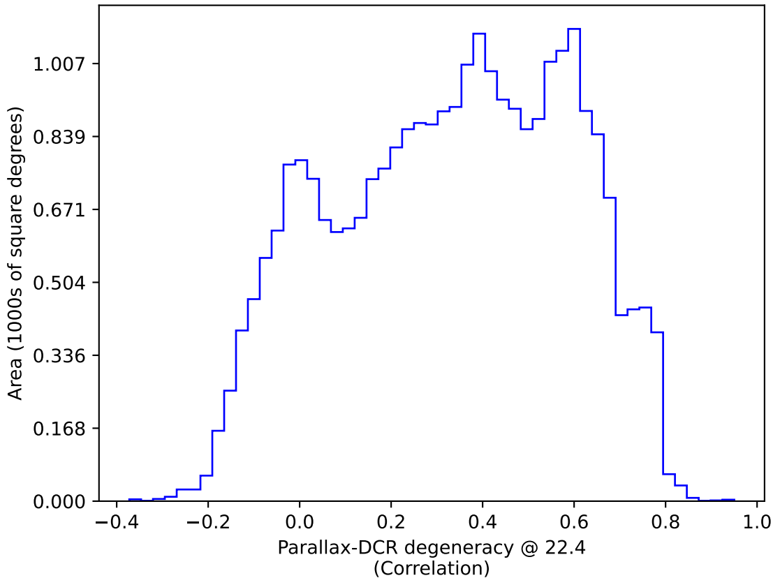
ddf_loaded_fl1_v3.4_10yrs : Parallax-DCR degeneracy @ 22.4
