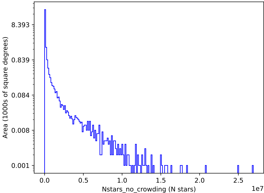
ddf_loaded_fl1_v3.4_10yrs z: Nstars_no_crowding
