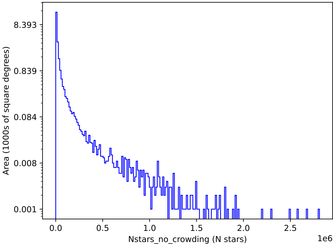
ddf_loaded_fl1_v3.4_10yrs u: Nstars_no_crowding
