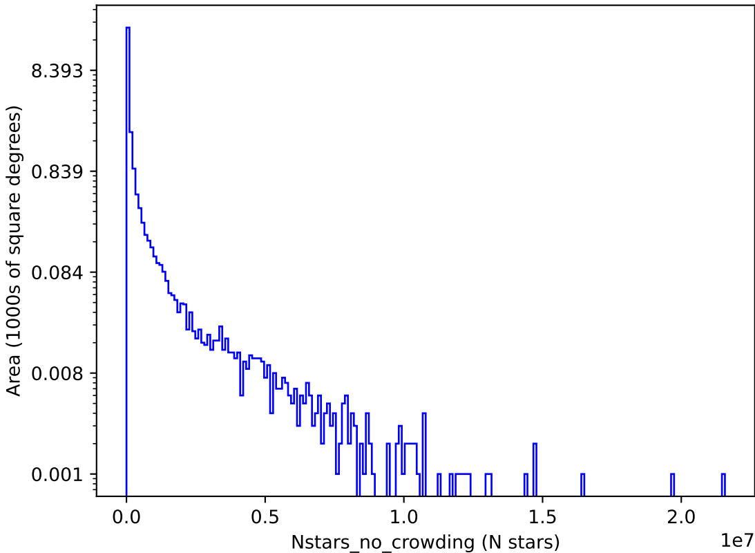
ddf_loaded_fl1_v3.4_10yrs r: Nstars_no_crowding
