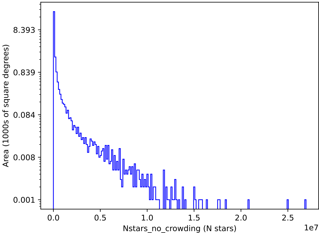
ddf_loaded_fl1_v3.4_10yrs i: Nstars_no_crowding
