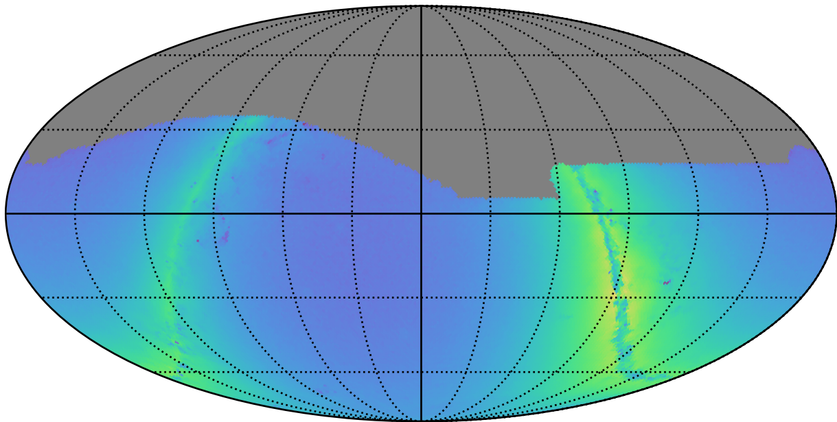
ddf_loaded_fl1_v3.4_10yrs g: Nstars_no_crowding
