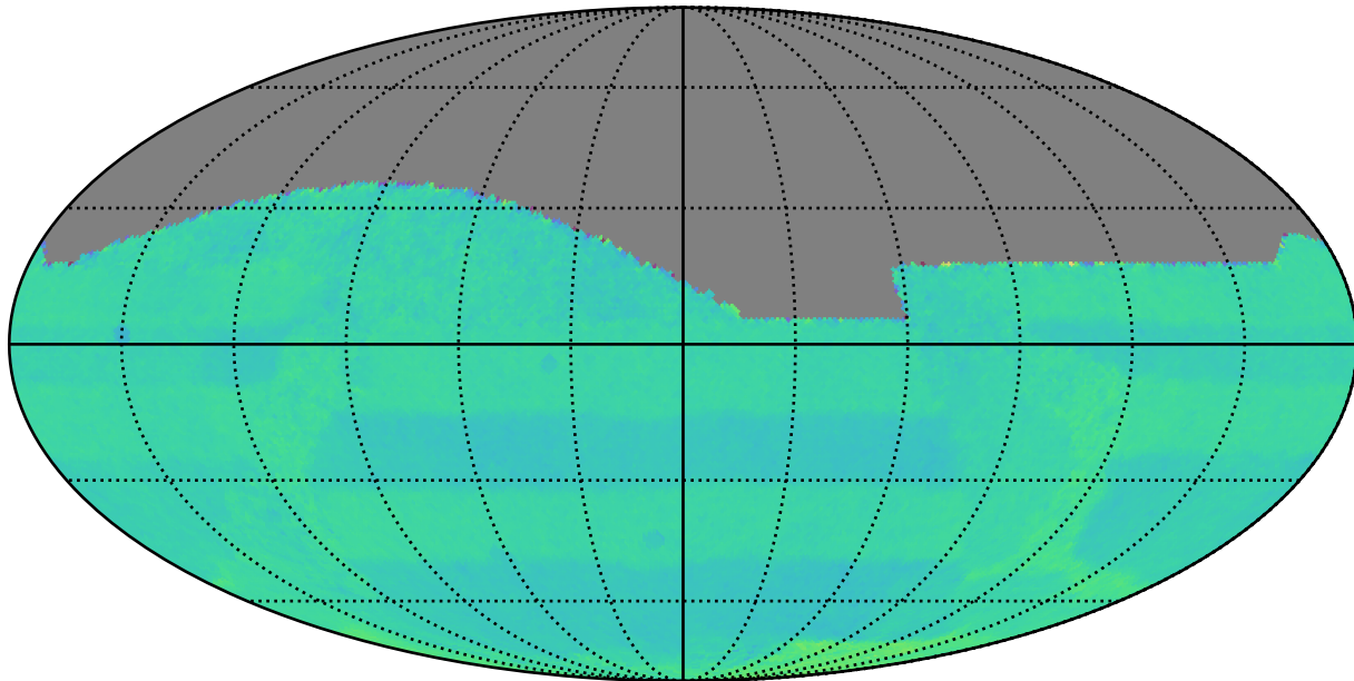
ddf_loaded_fl1_v3.4_10yrs : Normalized Proper Motion Uncert @ 20.5
