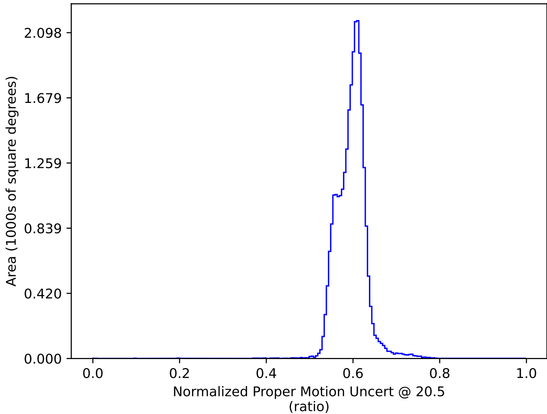
ddf_loaded_fl1_v3.4_10yrs : Normalized Proper Motion Uncert @ 20.5
