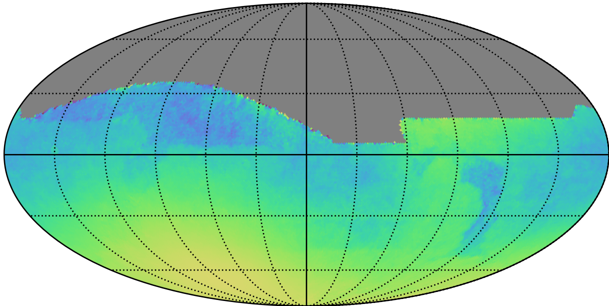
ddf_loaded_fl1_v3.4_10yrs : Normalized Parallax Uncert @ 24.0
