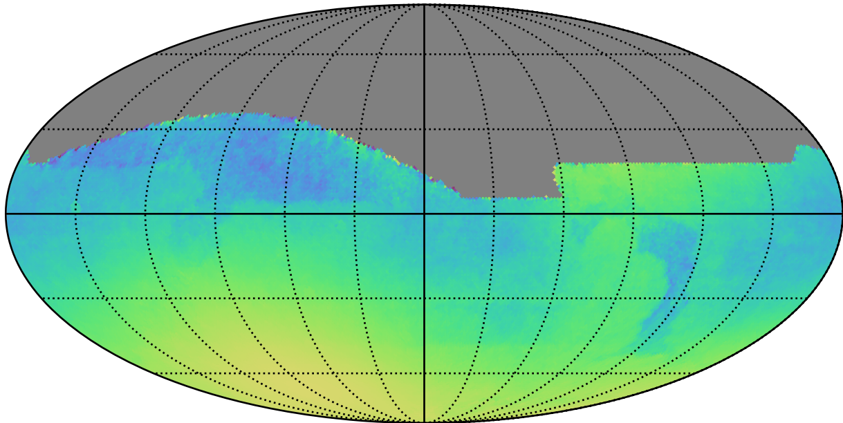
ddf_loaded_fl1_v3.4_10yrs : Normalized Parallax Uncert @ 22.4
