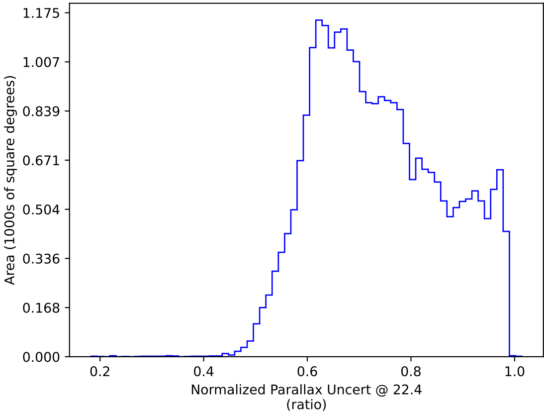
ddf_loaded_fl1_v3.4_10yrs : Normalized Parallax Uncert @ 22.4
