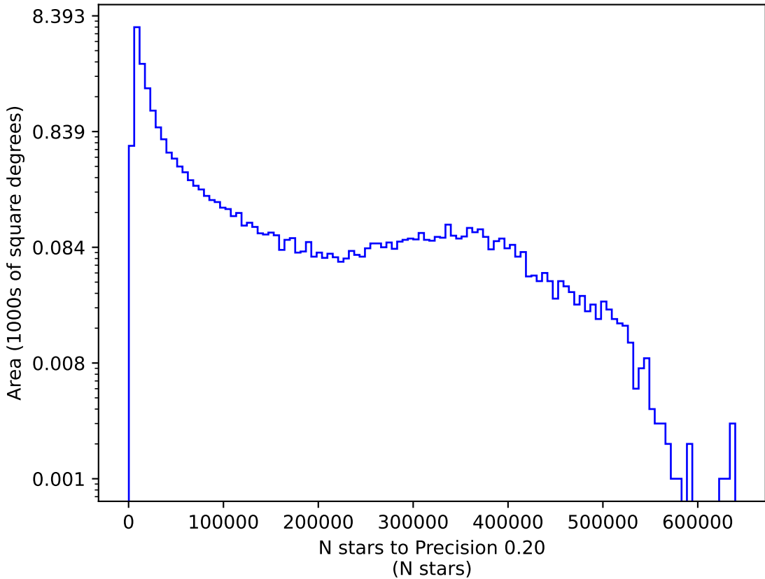
ddf_loaded_fl1_v3.4_10yrs y: N stars to Precision 0.20
