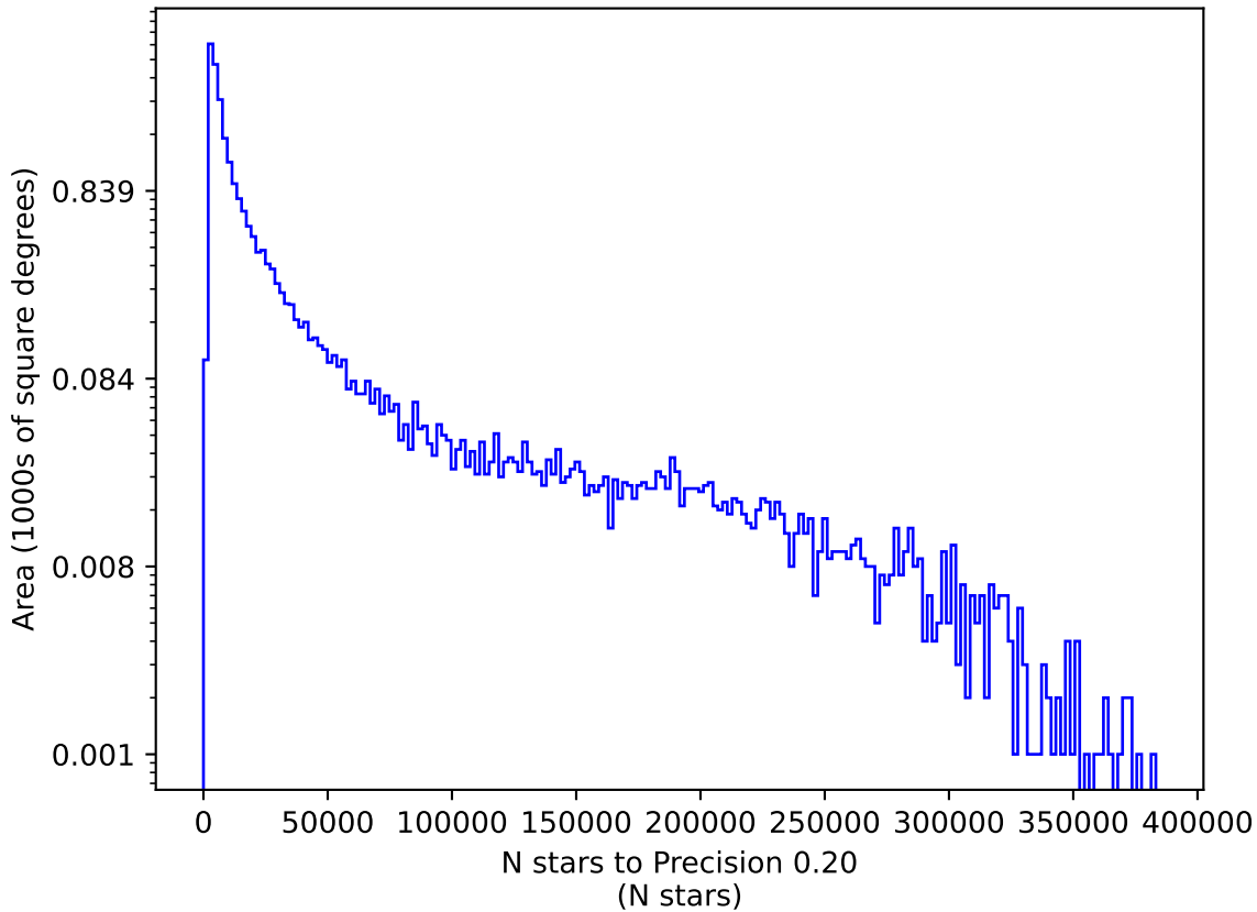
ddf_loaded_fl1_v3.4_10yrs u: N stars to Precision 0.20
