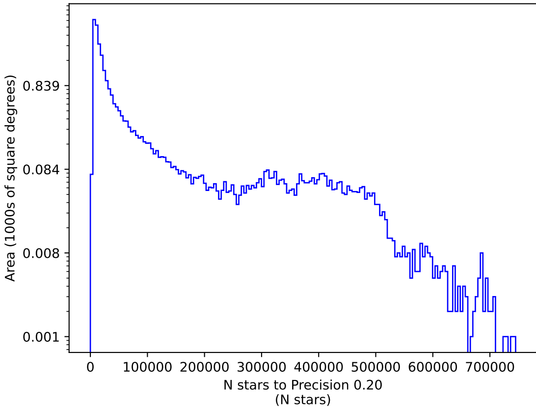
ddf_loaded_fl1_v3.4_10yrs r: N stars to Precision 0.20
