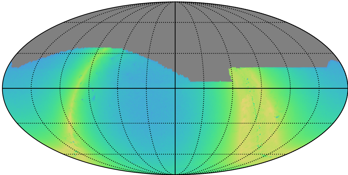
ddf_loaded_fl1_v3.4_10yrs i: N stars to Precision 0.20
