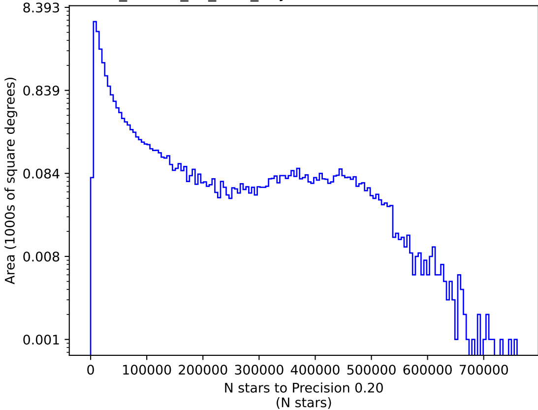
ddf_loaded_fl1_v3.4_10yrs i: N stars to Precision 0.20
