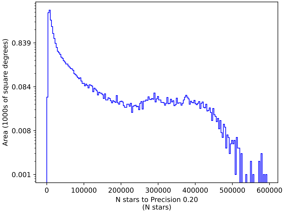
ddf_loaded_fl1_v3.4_10yrs g: N stars to Precision 0.20
