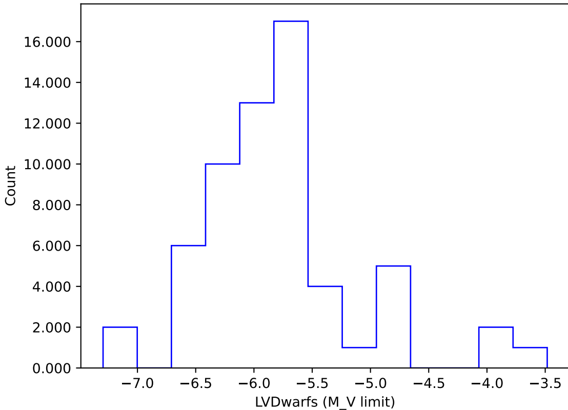
ddf_loaded_fl1_v3.4_10yrs gi: LVDwarfs
