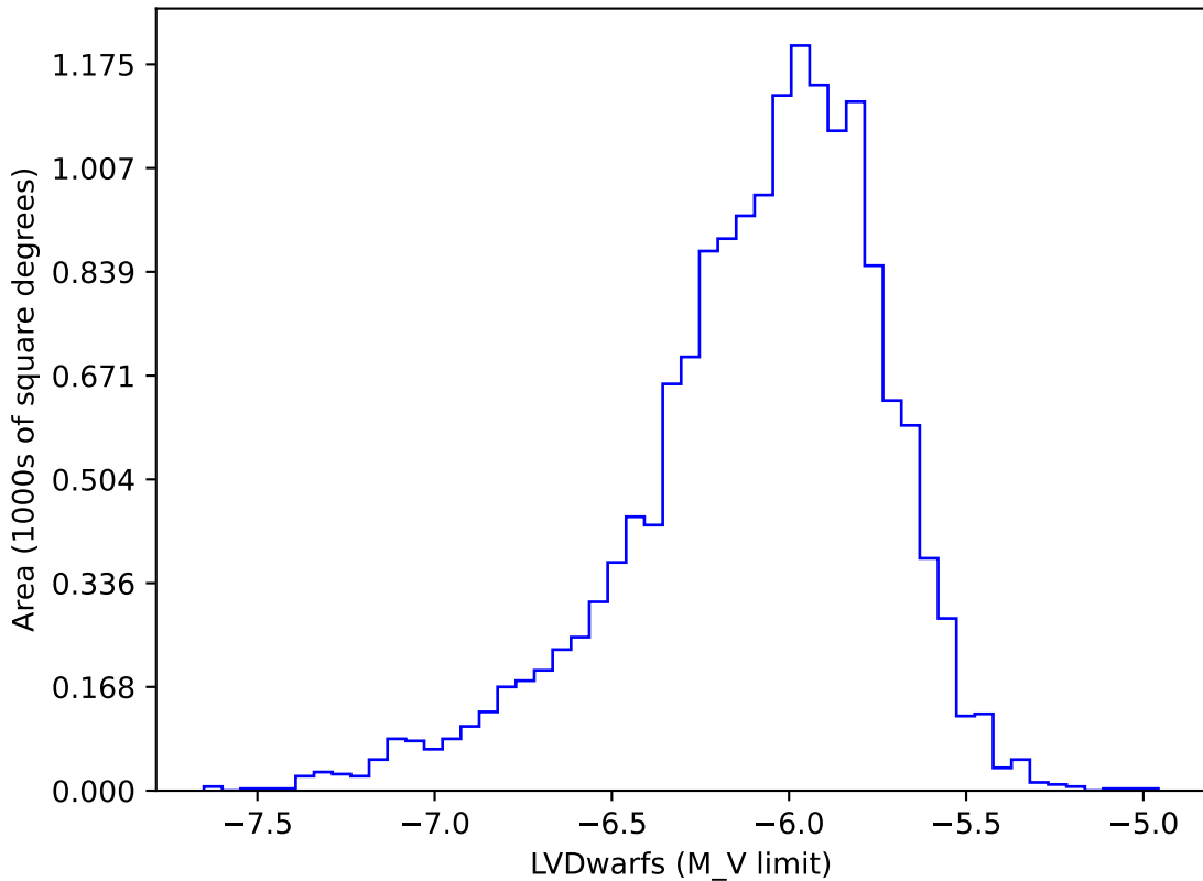
ddf_loaded_fl1_v3.4_10yrs gi: LVDwarfs
