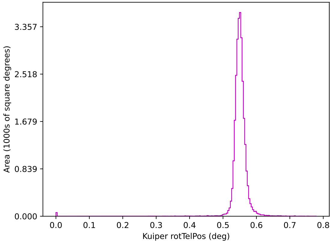
ddf_loaded_fl1_v3.4_10yrs z: Kuiper rotTelPos
