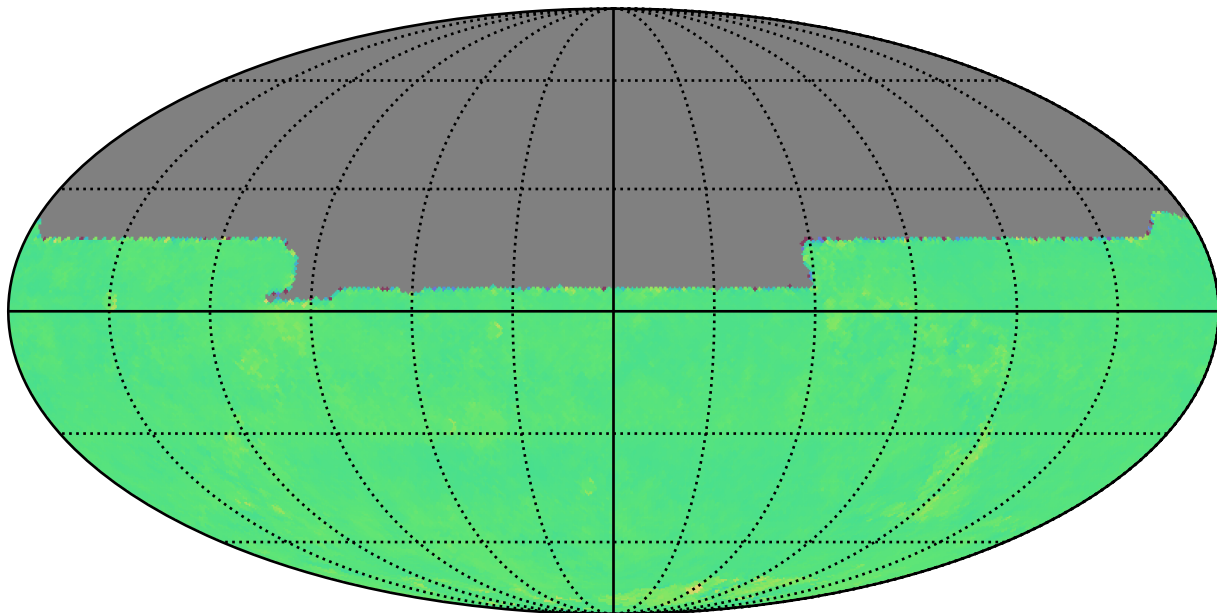
ddf_loaded_fl1_v3.4_10yrs y: Kuiper rotTelPos
