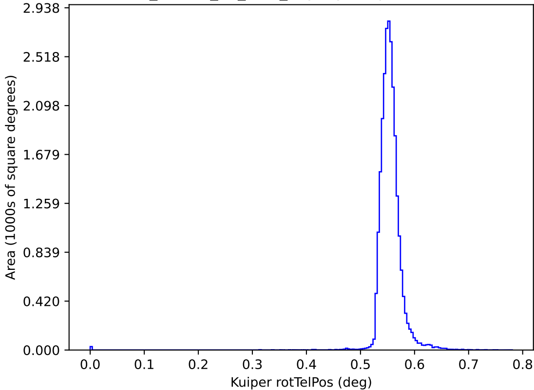
ddf_loaded_fl1_v3.4_10yrs y: Kuiper rotTelPos
