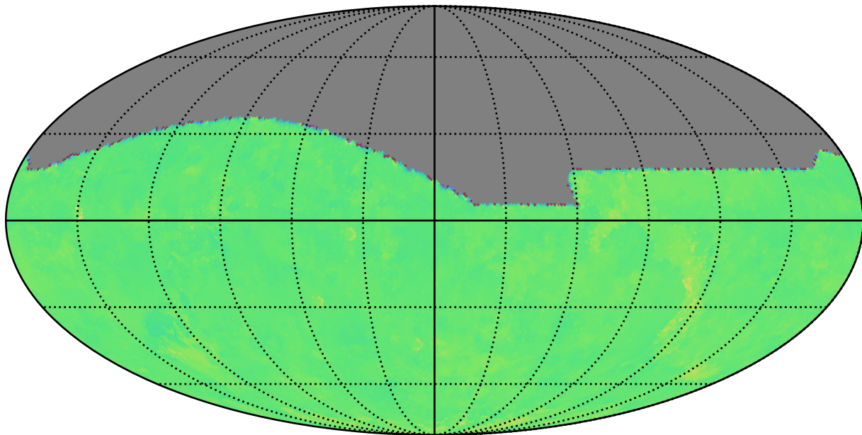
ddf_loaded_fl1_v3.4_10yrs g: Kuiper rotTelPos
