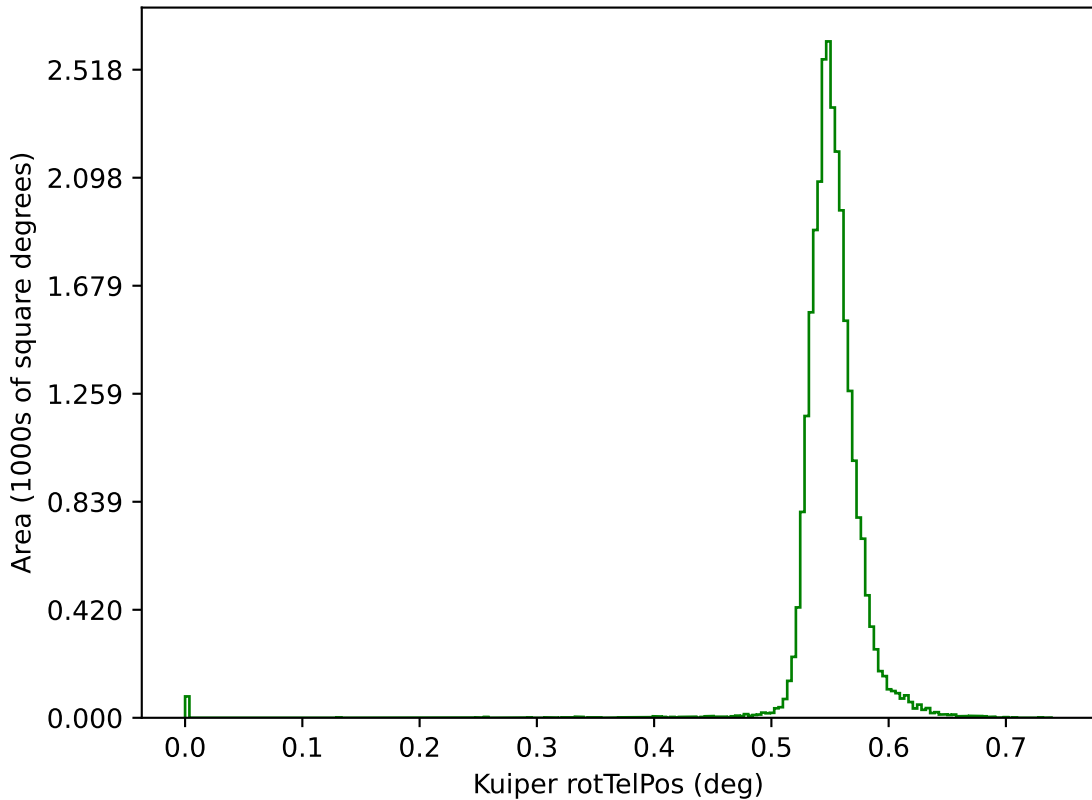
ddf_loaded_fl1_v3.4_10yrs g: Kuiper rotTelPos
