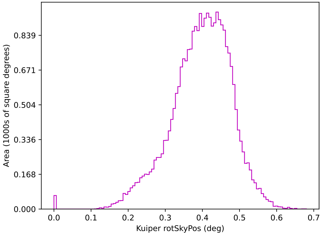
ddf_loaded_fl1_v3.4_10yrs z: Kuiper rotSkyPos
