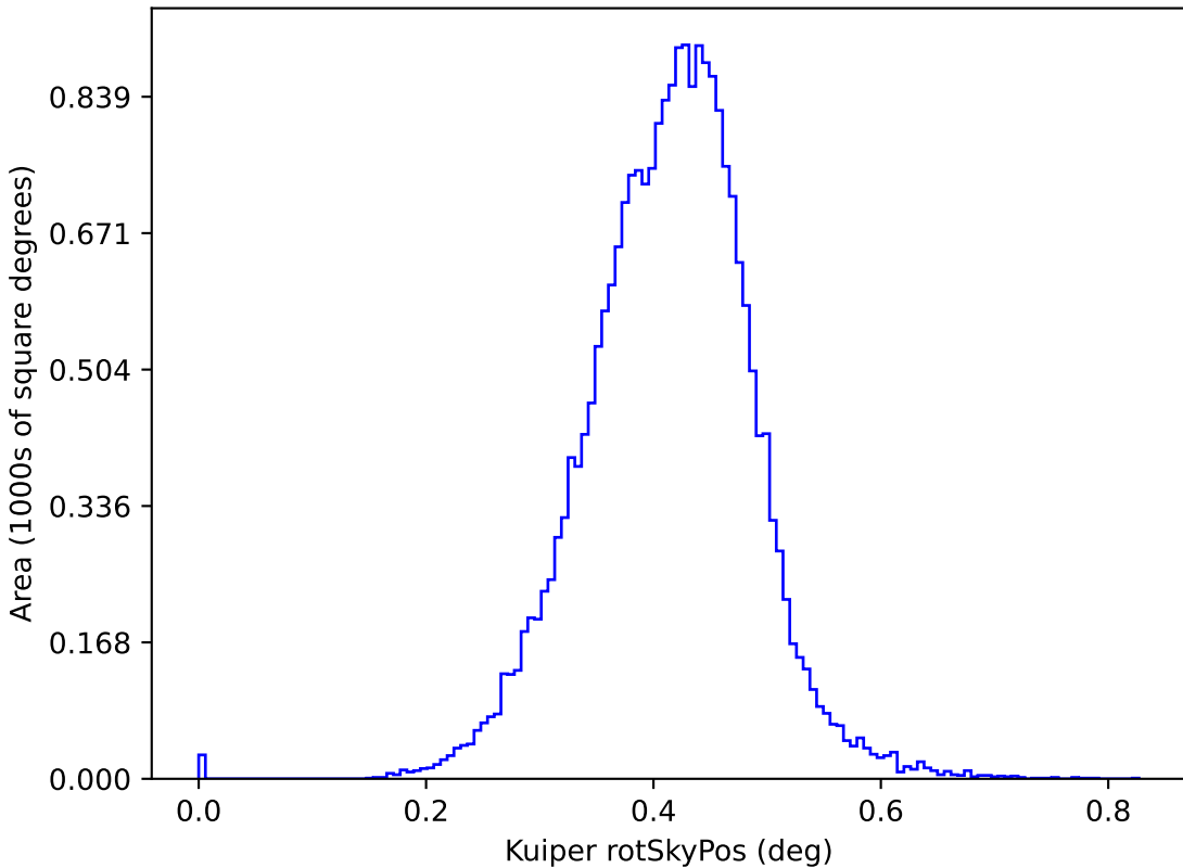
ddf_loaded_fl1_v3.4_10yrs y: Kuiper rotSkyPos
