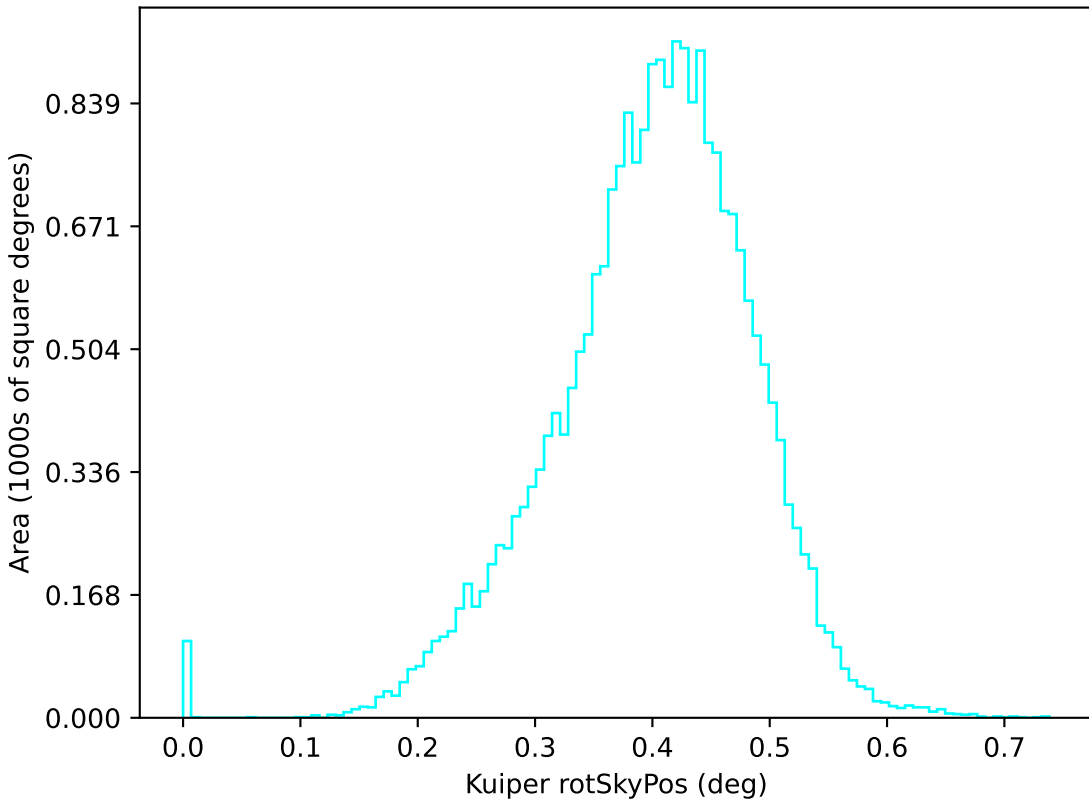
ddf_loaded_fl1_v3.4_10yrs u: Kuiper rotSkyPos
